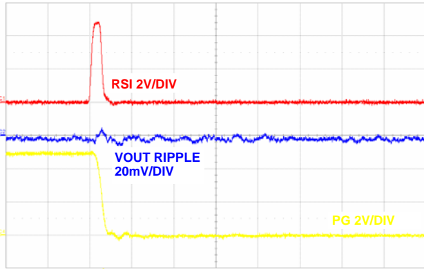
FIGURE 27. RSI RESET, (200µs/DIV)
