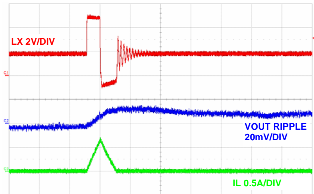
FIGURE 16. STEADY STATE OPERATION AT NO LOAD (PFM), (1μs/DIV)
