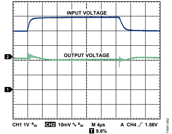
Figure 58. Line Transient Response, C_{IN} = C_{OUT} = 1 \mu F , I_{LOAD} = 1 \text{ mA} , V_{OUT} = 3.3 \text{ V}
