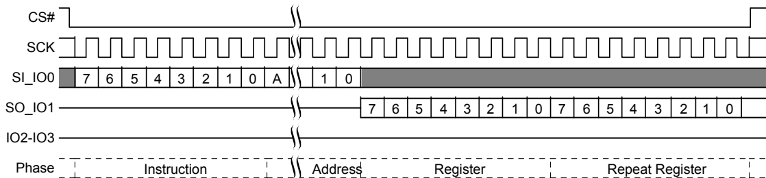
Figure 11.66 PPB Read Command Sequence
