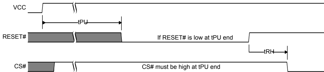
Figure 6.4 Reset low at the end of POR
