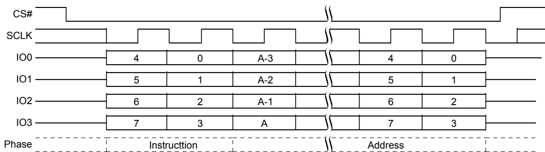
Figure 11.54 EES QPI Mode Command Sequence
