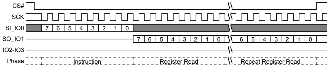
Figure 11.12 Read Configuration Register (RDCR) Command Sequence
