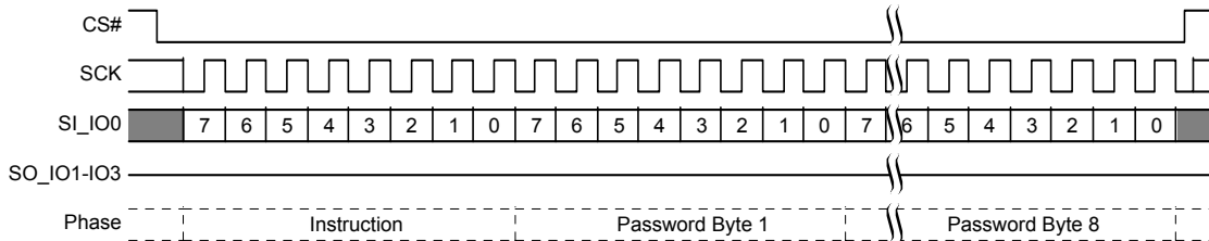
Figure 11.72 Password Program (PASSP) Command Sequence
