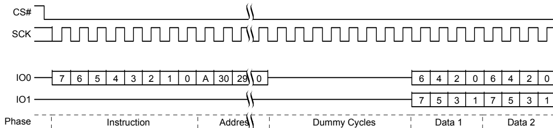
Figure 11.34 Dual Output Read Command Sequence
