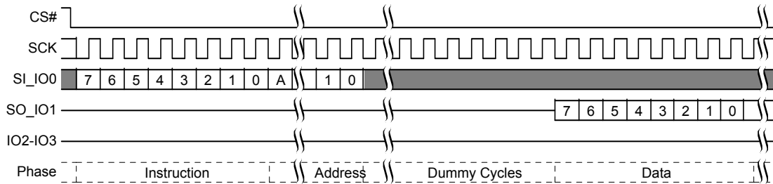
Figure 11.28 Read Any Register Read Command Sequence
