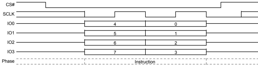
Figure 11.27 Enter 4 Byte Address QPI Mode
