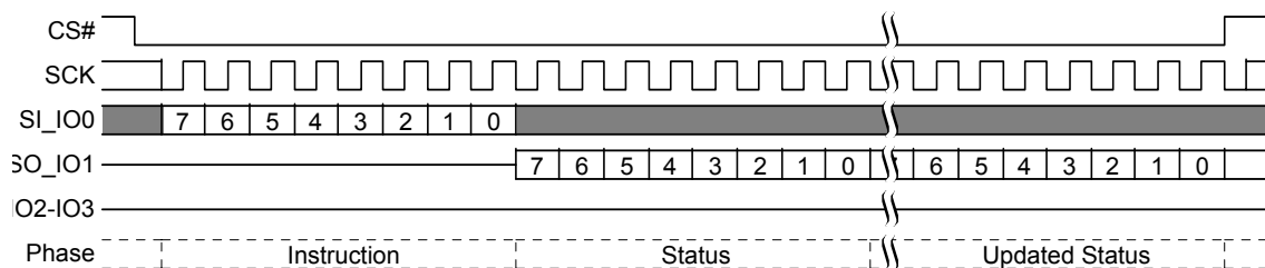
Figure 11.11 Read Status Register-2 (RDSR2) Command
